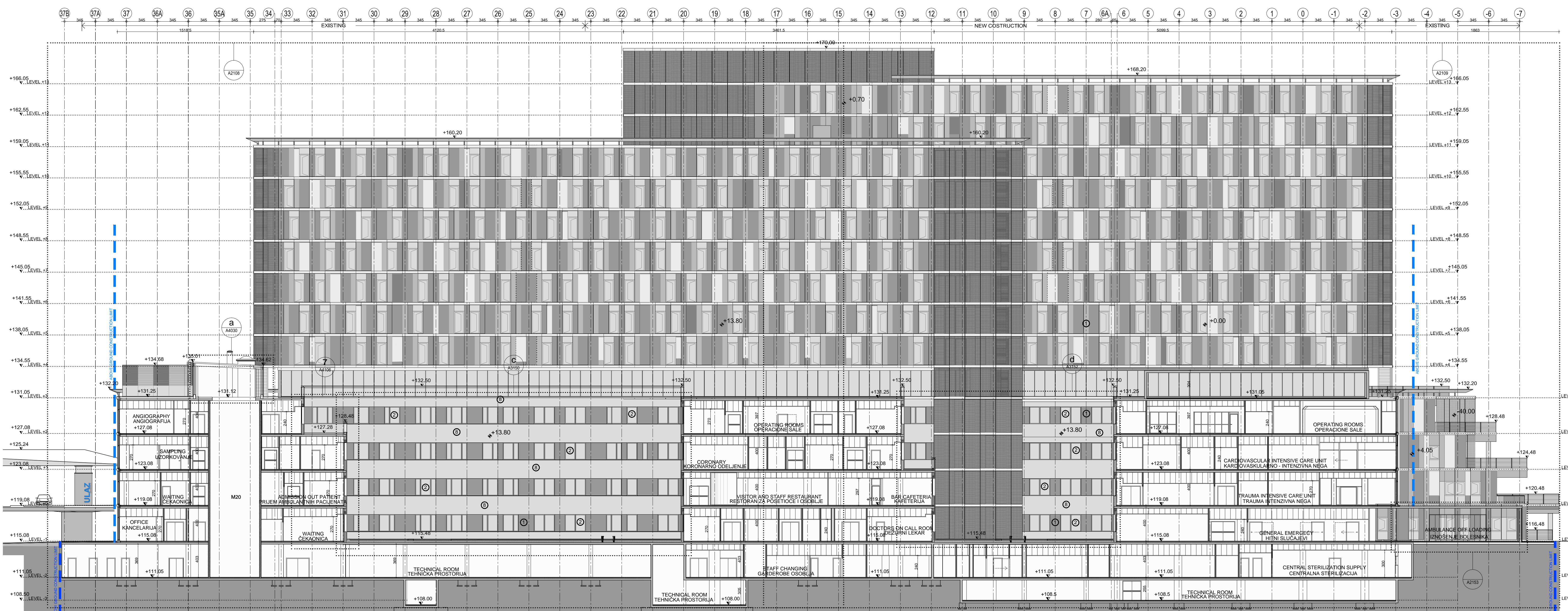
SECTION D PRESEK D
